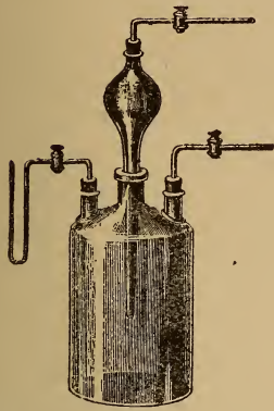
Fig. 100. WOULFF'S BOTTLE, FOR MAKING OXYGEN.
